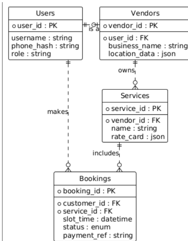
Figure 4.1: Entity Relationship Diagram (ERD) for the core data model.
