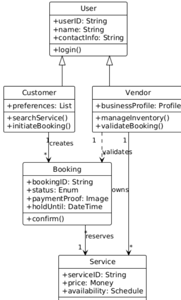
Figure 4.3: Class diagram for major domain objects and relationships.
