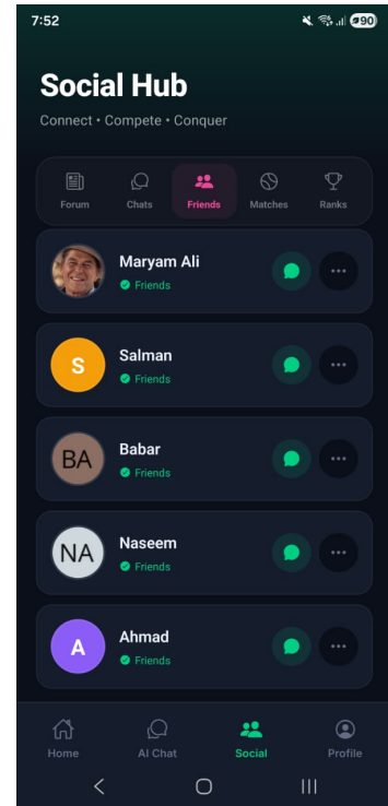
Figure 3.8: Friends list.
